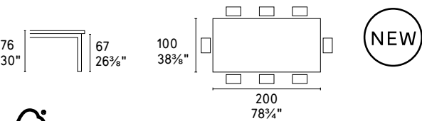
CS/4096-RC 200 C
