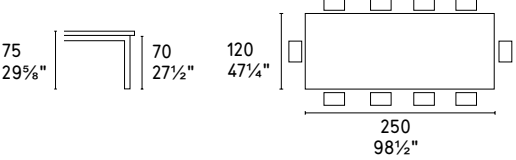
CS/4092-RL B 250
