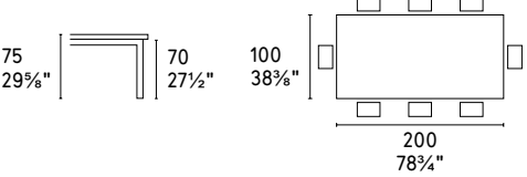
CS/4092-RL B 200
